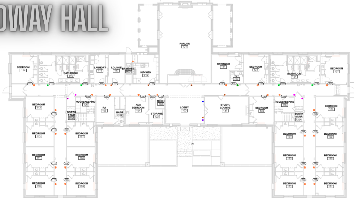
FIRST FLOOR
